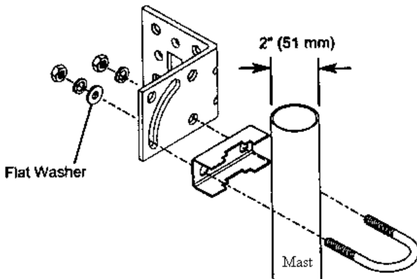
Configured for Vertical Polarity
